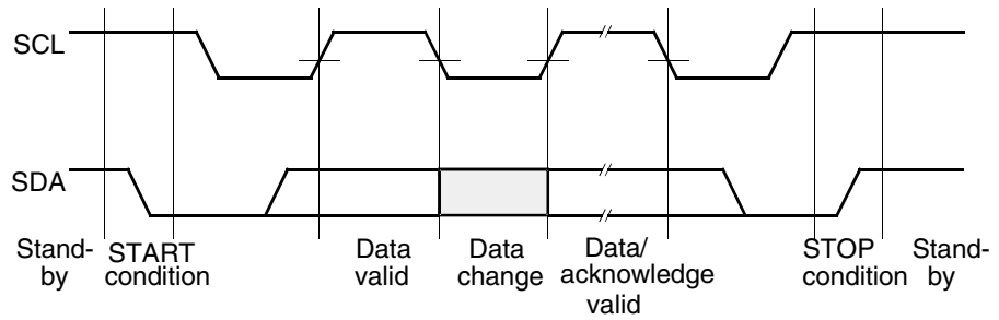
Figure 4-4. Serial Protocol
